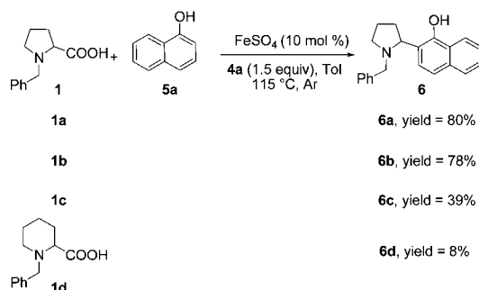
Scheme 1. Decarboxylative Coupling of \alpha -Naphthol
